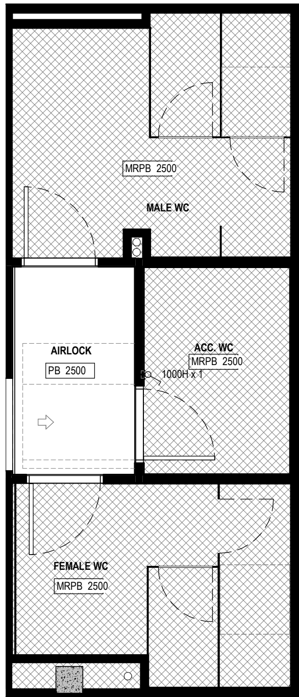
2 RCP - VILLAGE LIFESTYLE - AMENITIES Scale 1: 50
